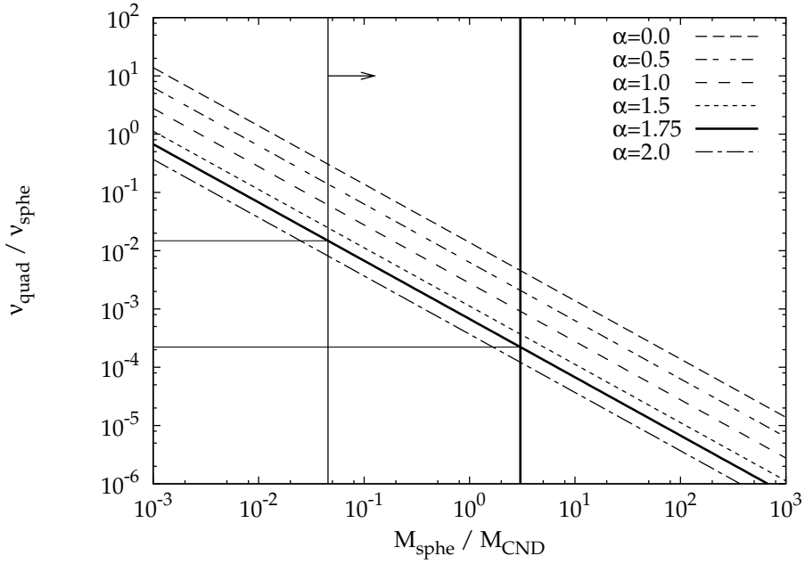
Figure 2.6: v_{\text{quad}}/v_{\text{sph}} for a test particle with a = 0.24 pc as a function of M_{\text{sph}}/M_{\text{CND}} and \alpha . The thick vertical line represents M_{\text{sph}}/M_{\text{CND}} according to current observations, while the thin vertical line with arrow represents M_{\text{sph}}/M_{\text{CND}} = 1/22 , the lower limit of the M_{\text{sph}}/M_{\text{CND}} ratio interval for which \omega circulates through the whole [0^\circ; 360^\circ] range.
