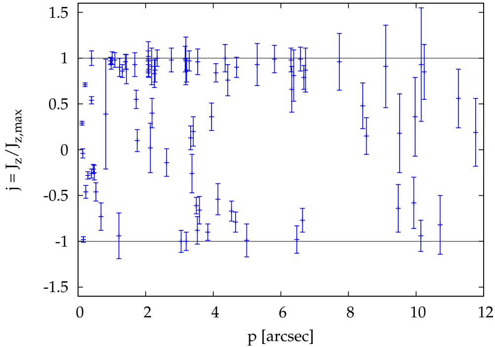
Figure 3.5: Distribution of the projected and normalized angular momentum on the sky j = J_z / J_{z, \max} (3.10) for the early-type stars as a function of the projected separation p from Sgr A* (for p > 0.08'' ). In this diagram stars on projected tangential, clockwise orbits are at j \simeq +1 , while stars on the tangential, counter-clockwise orbits are at j \simeq -1 . Stars at j \simeq 0 are on projected radial orbits.
