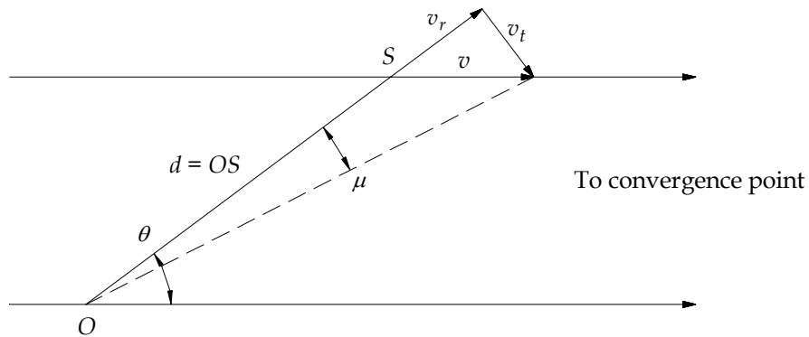
Figure 2.2: geometry of proper-motion and radial-velocity measurements.
