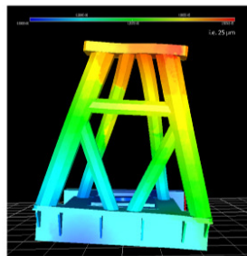
Figure 3: An optimisation of the alt-azimuth mount during the development phase. The final mount equipped with Officina Stellare RILA 600 f/5 reflector and a sensitive CCD camera (EZV chip 42-20-BI, >90% QE, FOV 0.52 deg). The complete autonomous observatory is now located in Ondřejov, Czech Republic. The first-light image (M31)!
