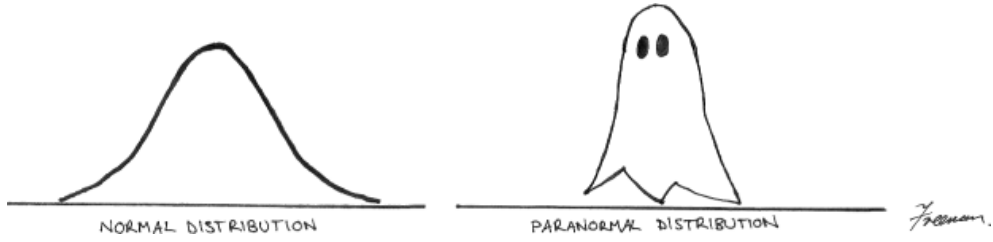
Figure 20: A normal distribution compared to a ‘paranormal’ one. A sketch we sometimes use to demonstrate the importance of thinking about uncertainties of observational data. Adapted from Freeman (2006).
