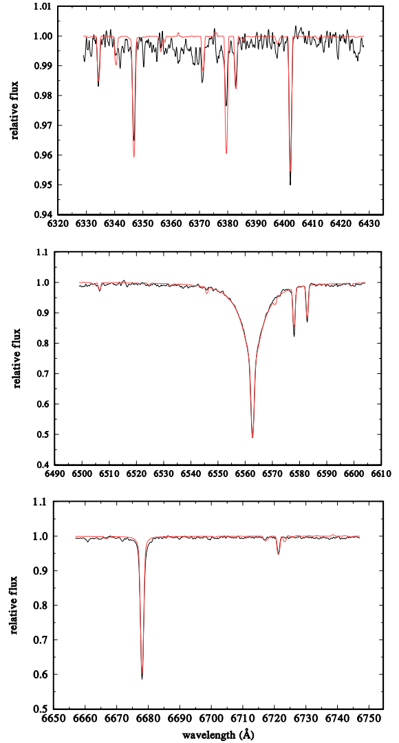
Fig. C.1. A comparison of the disentangled red spectrum of HD 31617 (black lines) with the model spectrum (red lines).
