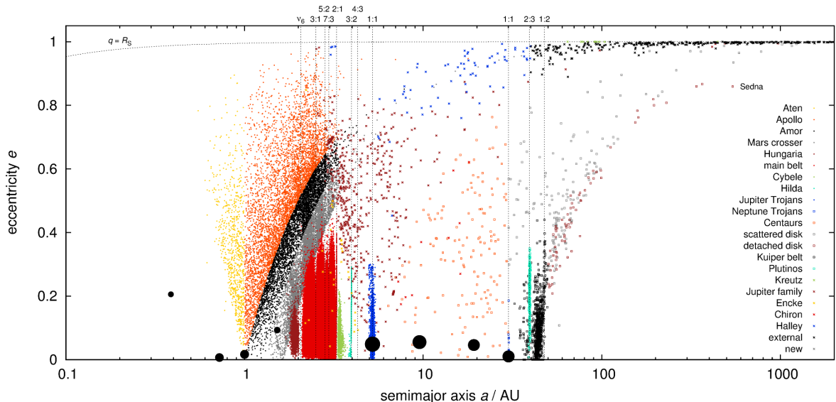
Figure 2: The observed state of the Solar System displayed on a plot the semimajor axis a vs the eccentricity e . Symbols and colours discriminate various types and populations of small bodies: asteroids are shown as circles, trans-neptunian objects as squares and comets as crosses. There are more than 5 \cdot 10^5 objects plotted, which might be either Aten, Apollo, Amor, Mars crosser, Hungaria, main belt asteroid, Cybele, Hilda, Jupiter Trojan, Centaur, Neptune Trojan, scattered disk, detached disk, Kuiper belt, Plutino, Kreutz comet, Jupiter family, Encke, Chiron, Halley, external, or new comet. Data were downloaded from the Minor Planet Center, AstOrb and AstDyS catalogues. Vertical lines denote major mean-motion resonances with Jupiter or Neptune and the \nu_6 secular resonance. The dotted line (close to the top) corresponds to the perihelion distance q equal to the radius R_\odot of the Sun.
