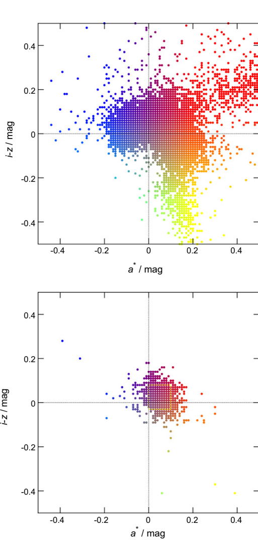
Fig. 1. Colour indices i - z and a^* (defined in Parker et al. (2008)) of all asteroids from the Sloan Digital Sky Survey, Moving Object Catalogue version 4 and the corresponding colour palette (top panel) which is used in the following figures to distinguish colours of asteroids. We also plot the Eos family members observed by the SDSS (bottom panel) with small photometric uncertainties (less than 0.03 mag). The inferred range of colour indices (denoted by the dashed yellow rectangle) is then used as a criterion for the selection of the Eos-like asteroids in the broad surroundings of the nominal family. The rectangle does not encompass the outliers. (For interpretation of the references to colour in this figure legend, the reader is referred to the web version of this article.)
