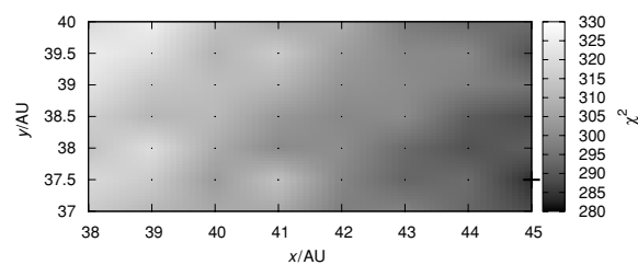
Figure 8. Minima of the seven-dimensional function \chi^2(m_4, x_{h4}, y_{h4}, z_{h4}, v_{xh4}, v_{yh4}, v_{zh4}) at given positions (x_{h4}, y_{h4}) . The minimum is taken over remaining free parameters m_4, z_{h4}, v_{xh4}, v_{yh4}, v_{zh4} . Cross is an overall minimum and black dots represent computed points.
