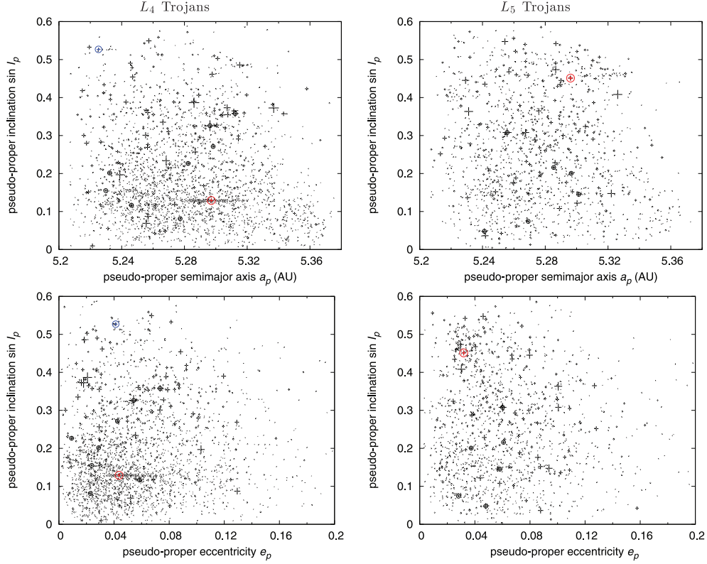
Figure 2. The resonant elements ( a \equiv \bar{a} + d , \sin I ) and ( e , \sin I ) for L_4 and L_5 Trojans. The crosses indicate relative sizes of bodies, taken either from the AstOrb catalogue or computed from absolute magnitude H and geometric albedo p_V . In this plot, we assumed p_V = 0.058 for L_4 Trojans and 0.045 for those in L_5 (it corresponds to medians of known p_V s). The asteroids (3548) Eurybates in L_4 and (4709) Ennomos in L_5 , around which significant clusters are visible, are shown in red. Moreover, the asteroid (9799) 1996 RJ in L_4 , which is surrounded by a small cluster, is denoted by a blue circle. [This cluster is so tight that its members are located inside the circle on the ( e , \sin I ) plot.]
