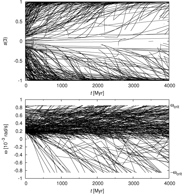
Figure 6. An example of the YORP-driven evolution of obliquities (namely a z -component of the spin-axis unit vector, top panel) and angular velocities \omega (bottom panel) for the members of the synthetic ‘Hilda’ family. At the beginning, all values of \omega were selected positive and spin axes were distributed isotropically. The evolution may force \omega to become negative, which simply corresponds to an opposite orientation of the spin axis. The scaling parameter selected for this run was c_{\text{YORP}} = 0.33 .
