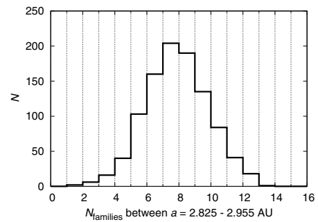
Fig. 13. Histogram for the expected number of LHB families located in the “pristine zone” of the main belt.
