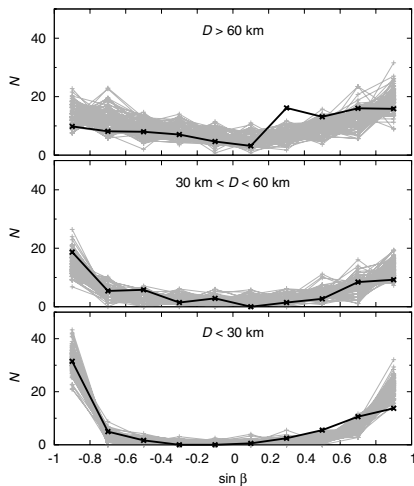
Fig. 12. Steady-state synthetic latitude distributions for three different size ranges: D > 60 km (top), 30 \text{ km} < D < 60 km (middle) and D < 30 km (bottom). The synthetic distributions are plotted by thin gray lines while the observed distribution by a thick black line.
