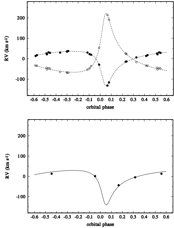
Fig. 2. Orbital radial-velocity curves of HD 31894 for the orbital period of 11 d 0459. Phase zero corresponds to the superior conjunction. Upper panel: RV curves of the primary (filled circles) and secondary (open circles) and the PHOEBE solution calculated curves. Bottom panel: the RV curve based on the old DAO RVs.
