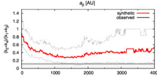
Figure 1: An example of the Flora family spin-orbital evolution: (a) the observed proper semimajor axis a_0 vs the absolute magnitude H , (b) a_0 vs pole latitude \beta , with sizes D denoted by symbols; (c) the same for a simulation of large asteroids ( D > 30 km); and (d) small asteroids. Finally, (e) a sort of x^2 metric vs time t .
