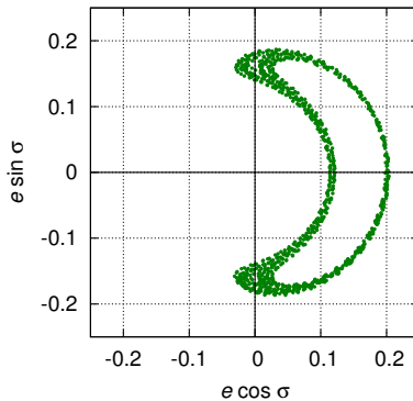
Figure 3: A typical trajectory of an asteroid located inside the 2:1 mean-motion resonance with Jupiter on a polar plot the eccentricity e vs the critical angle \sigma , as defined by Eq. (1). The angle \sigma exhibits librations in this case, not circulations about the origin.
