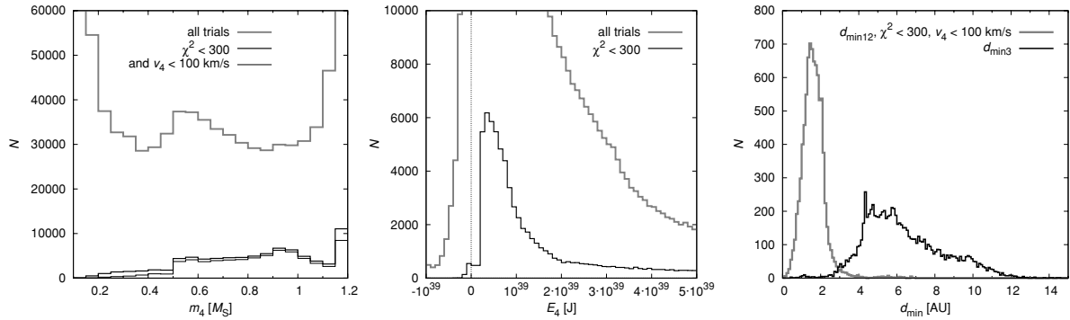
Figure 11. Left: histogram of masses m_4 of all trials and good ones (with \chi^2 < 300 and the lower absolute value of velocity |v_4| < 100 km s ^{-1} ). Middle: histogram of total energies E_4 of the fourth body at the epoch T_0 . There is a strong preference for hyperbolic orbits ( E_4 > 0 ), but one can find approximately 1% of orbits with negative energies. Right: histogram of minimum distances d_{\min 1+2} , d_{\min 3} of the fourth body from the (1+2) and third body (only good trials are shown). According to these distributions, it is more likely that the fourth body approached the (1+2) body closer than the third body. Median values are d_{\min 1+2} = 1.6 AU and d_{\min 3} = 5.9 AU.
