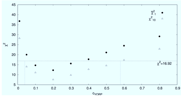
Fig. 6. Dependence of \bar{\chi}_t^2 and \chi_{10}^2 values calculated for the time t = 4 Gyr (i.e. the final state of the simulation) on different values of the c_{YORP} parameter. We also plotted the statistically significant probability value of 5% which corresponds to \chi^2 = 16.92 and the interval of plausible c_{YORP} values from 0.05 to 0.6.
