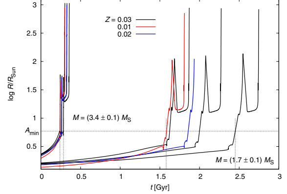
Figure 14. Evolution of radii for stars with different masses ( M = 1.6, 1.7, 1.8, and 3.3, 3.4, 3.5 M_\odot , Z = 0.03 ) and metallicities ( M = 1.7 and 3.4 M_\odot , Z = 0.01, 0.02 ). This computation was performed by the program EZ (Paxton 2004). The upper limit for the age of the second component is then 1.5–2.5 Gyr, while the lower limit is between 0.24 and 0.29 Gyr.
