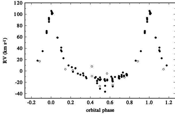
Fig. 3. The radial-velocity curve of the primary component of V2368 Oph based on H\alpha RVs measured in SPEFO for our OND, DAO, and SPM spectra (filled circles) and published RVs (open circles) for the period of 38^d.3307 from the FOTEL orbital solution with phase zero at periastron passage. See the text for details.
