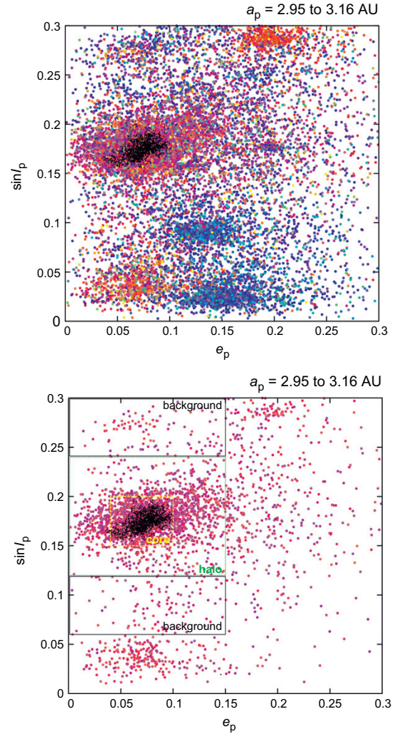
Fig. 2. The proper eccentricity e_p vs proper inclination \sin I_p plot for asteroids included in the SDSS MOC 4 catalogue. The proper semimajor axis is confined to the interval 2.95–3.16 AU, i.e. the Eos family zone. Colour coding corresponds to the SDSS colour indices according to Fig. 1. The top panel includes all asteroids (regardless of their colours). The bottom panel shows only a subset of 'Eos-like' asteroids with colours similar to those of the Eos members (see Fig. 1, bottom). Moreover, we denote a box used for the definition of the family 'core' (dashed yellow line) a larger box for the 'halo' (dotted green line) and two boxes considered as 'background' (thin black line). For comparison, we also plot positions of the nominal Eos family members (black dots), identified for the velocity v_{\text{cutoff}} = 50 m/s. (For interpretation of the references to colour in this figure legend, the reader is referred to the web version of this article.)
