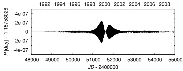
Figure 3. Simulated oscillating orbital period P of the central binary (bodies 1 and 2), perturbed by the third body. The periastron passage occurred in 2000 and the corresponding change of period is \Delta P \lesssim 10^{-7} days. The observed values of |\Delta P| \simeq 10^{-5} days are much larger than in this simulation.
