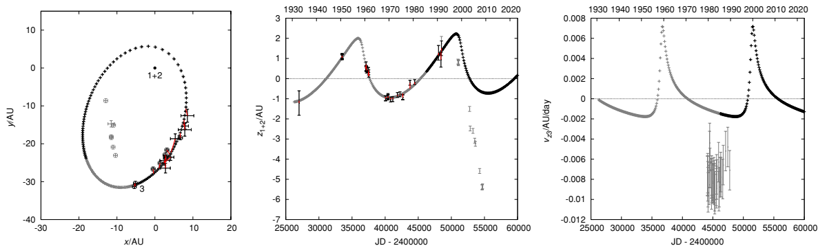
Figure 5. Best-fit solution for the orbit of the third body and the light-time effect before 2000: d = 102 pc, m_3 = 1.2 M_{\odot} , z_{h3} = 4.0 AU, v_{xh3} = 0.0036 AU day ^{-1} , v_{yh3} = 0.0013 AU day ^{-1} , v_{zh3} = -0.0015 AU day ^{-1} for T_0 = 2446282.24375 JD. The resulting \chi^2 = 88 , with the total number of data points N = 46 . The red lines denote differences between observed and calculated data. Radial velocities were not fitted in this case; they are shown for comparison only.
