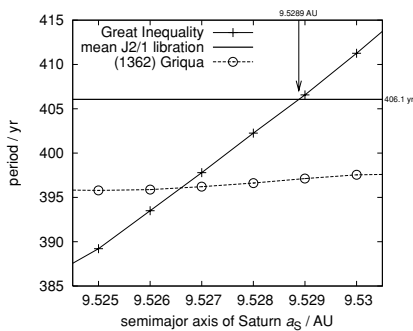
Figure 22. Dependence of the period associated with circulation of the GI angle 5\lambda_S - 2\lambda_J ( \lambda_S and \lambda_J are mean longitude in orbit for Saturn and Jupiter) on the osculating semimajor axis a_S of Saturn (crosses); Jupiter’s orbit is fixed. Moving Saturn farther away from the location of 2:5 resonance with Jupiter (at a_S = 9.584 au) makes the GI period shorter (with today’s a_S = 9.5289 au the GI period is about 880 yr). In the interval of a_S values shown in this figure the GI period becomes comparable to the average period \bar{P}_{J2/1} of librations in the J2/1 resonance (solid line). Libration period for a particular case of asteroid (1362) Griqua is shown by circles.
