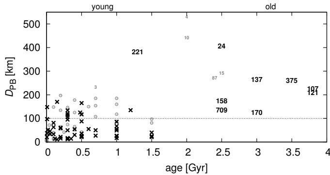
Figure 9: The relation between dynamical ages of families and the sizes D_{PB} of their parent bodies. Black crosses (or large labels) correspond to catastrophic disruptions, while cratering events are labelled by gray circles (small labels). Some of the families are denoted by the designation of the largest member. Adapted from Brož et al. (2013) and updated according to Nesvorný et al. (submitted).
