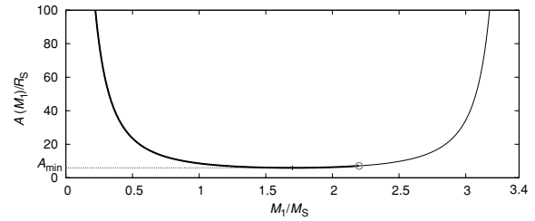
Figure 4. Dependence of separation A of the eclipsing binary on the mass M_1 of the first body, resulting from the conservation of total mass and orbital angular momentum. The thick line denotes past evolution, the circle the current state M_1 = 2.2 M_\odot , and the thin line the future evolution.
