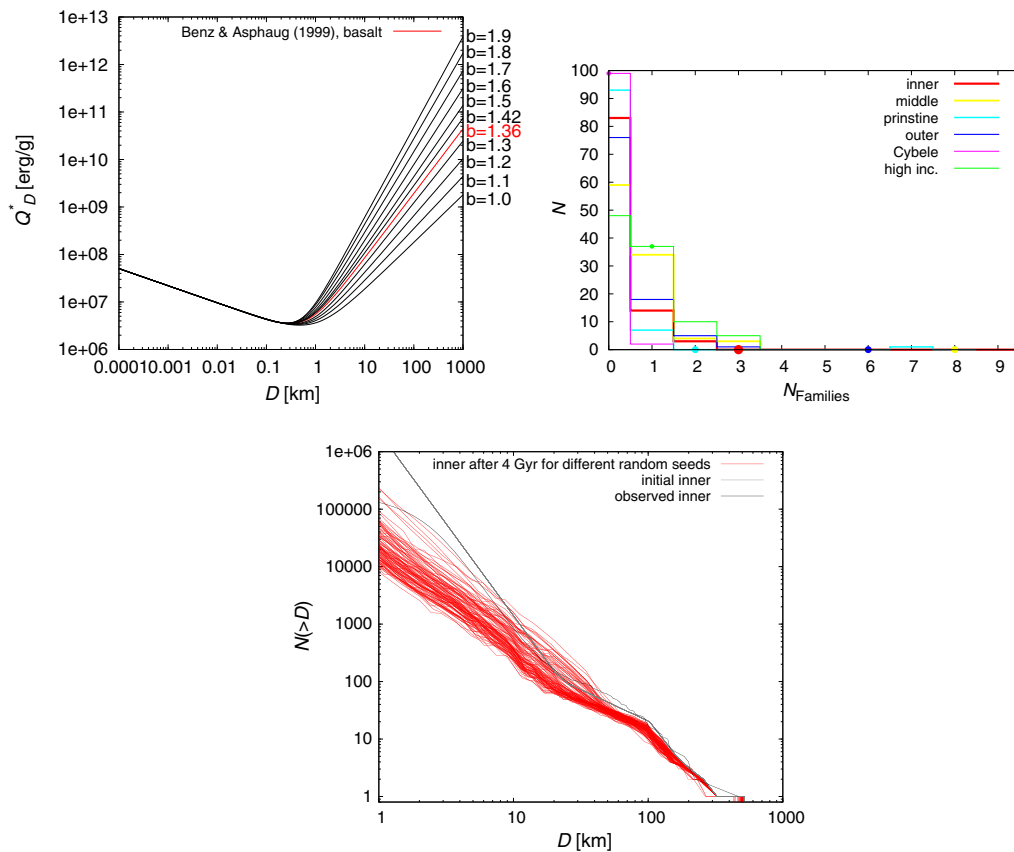
Fig. 17. Left: A number of scaling laws with modified strength of large bodies (a similar set as in Bottke et al. (2005) ). The red line represents the nominal scaling law of Benz and Asphaug (1999) . Middle: histograms representing the number N of simulations (out of 100) a given number of families N_{\text{families}} was created; we assumed the scaling law with an increased strength of large bodies ( b = 1.9 ). The observed numbers of families are displayed as filled circles for comparison. Right: the final size–frequency distributions of the inner belt for 100 simulations with different random seeds and for the scaling law with a decreased strength of large bodies ( b = 1.0 ). Neither of these two mentioned simulations is consistent with the observations (their \chi^2 would be clearly much larger than the best fit from Section 6). (For interpretation of the references to colour in this figure legend, the reader is referred to the web version of this article.)
