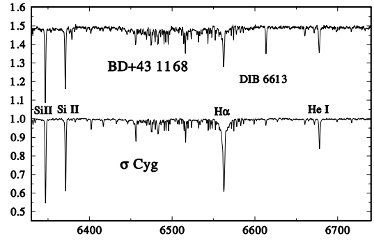
Fig. 8. A comparison of the Ondřejov red spectrum of BD+43° 1168 taken on HJD 2 456 008.3159 with a spectrum of another B9Iab star \sigma Cyg, taken with the same instrumentation and kindly put at our disposal by Dr. M. Kraus. Note the strong 6613.56 Å interstellar line in the spectrum of BD+43° 1168 and its faint H\alpha profile, obviously partly filled by emission.
