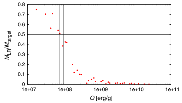
Fig. 9. The dependence of the mass of the largest remnant M_{\text{LR}} on the kinetic energy Q of the projectile for rubble-pile bodies. We mark the value M_{\text{LR}}/M_{\text{target}} = 0.5 with a horizontal line, according to this value we determine Q_D^* . The uncertainties of the determination of Q_D^* are denoted by vertical lines. The result is Q_D^* = (9 \pm 1) \times 10^7 \text{ erg g}^{-1} .
